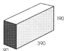
10.31 Solid - full length
