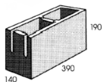
15.41 Closed end
