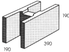
20.48 'H' block
