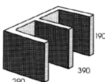
30.45 Clean-out stretcher
