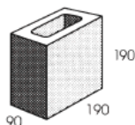
10.03 Hollow - half
