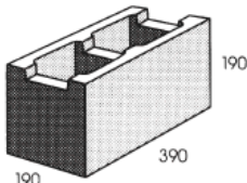
20.42 Notch Block
