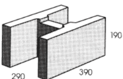
30.48 'H' block
