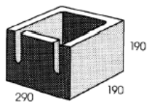
20.02/30.43 Hollow - half/ Closed end - half
