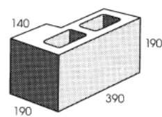
15.25 Hollow - corner return
