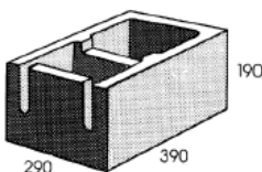
30.41 Closed end
