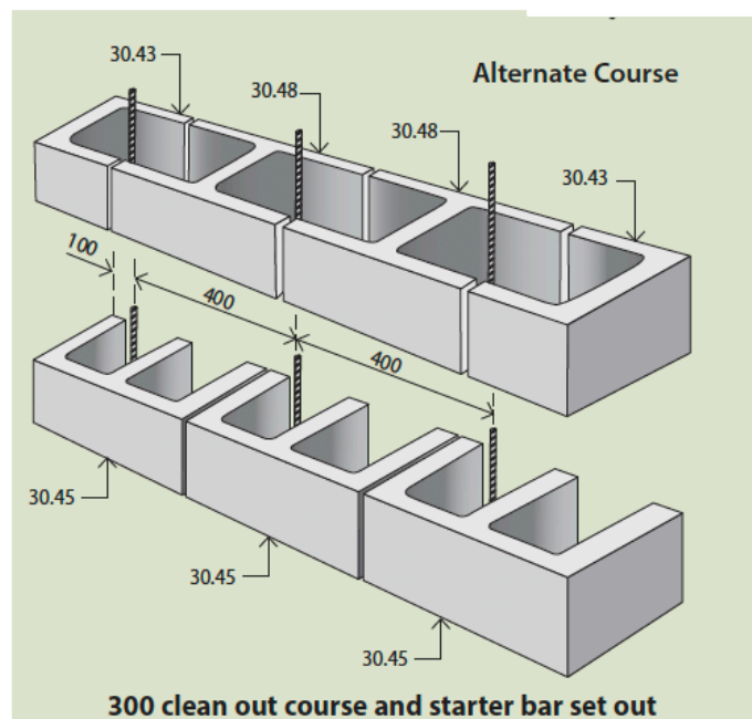
30.45 Clean-out stretcher
