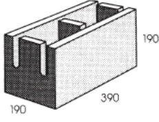
20.20 Knock-out bond beam
